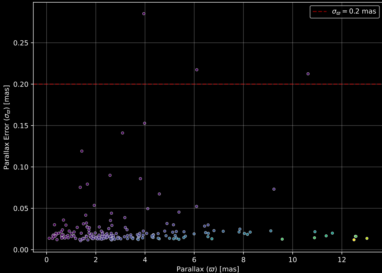
APOGEE DR17 Field: [165+33_MGA] Parallax Quality (n= 187)
