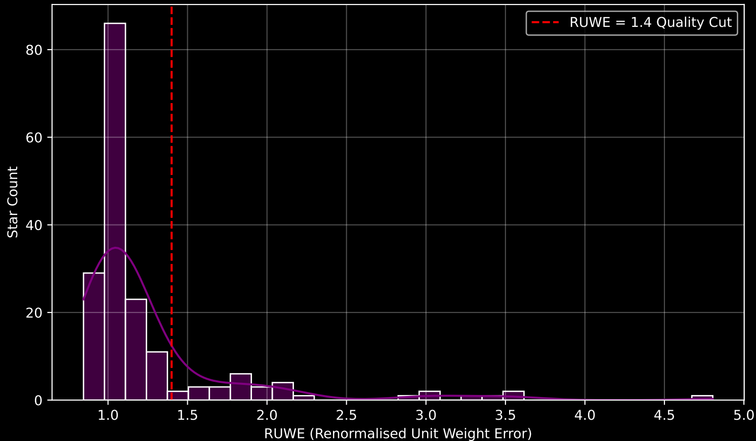
GAPOGEE DR17 Field [165+33_MGA] RUWE Distribution (n= 179)
