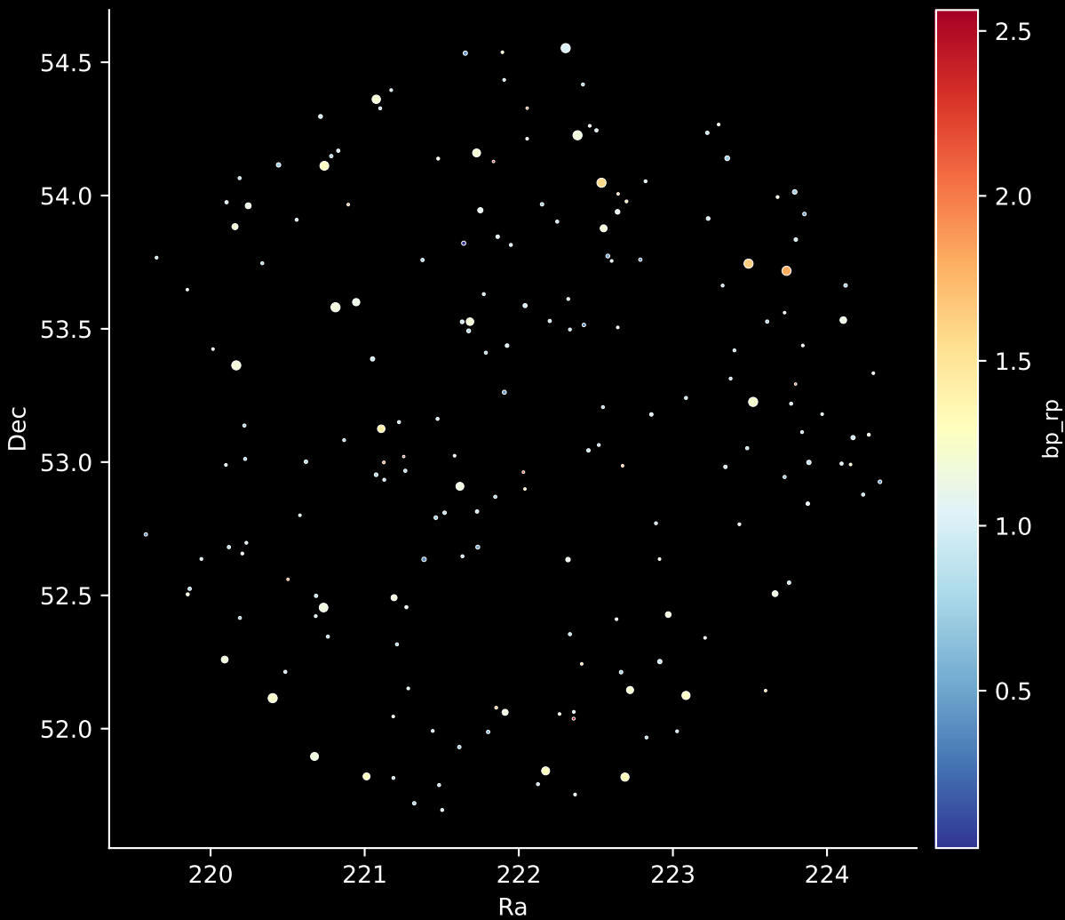
APOGEE DR17 Field: [165+33_MGA] Stars: 187
