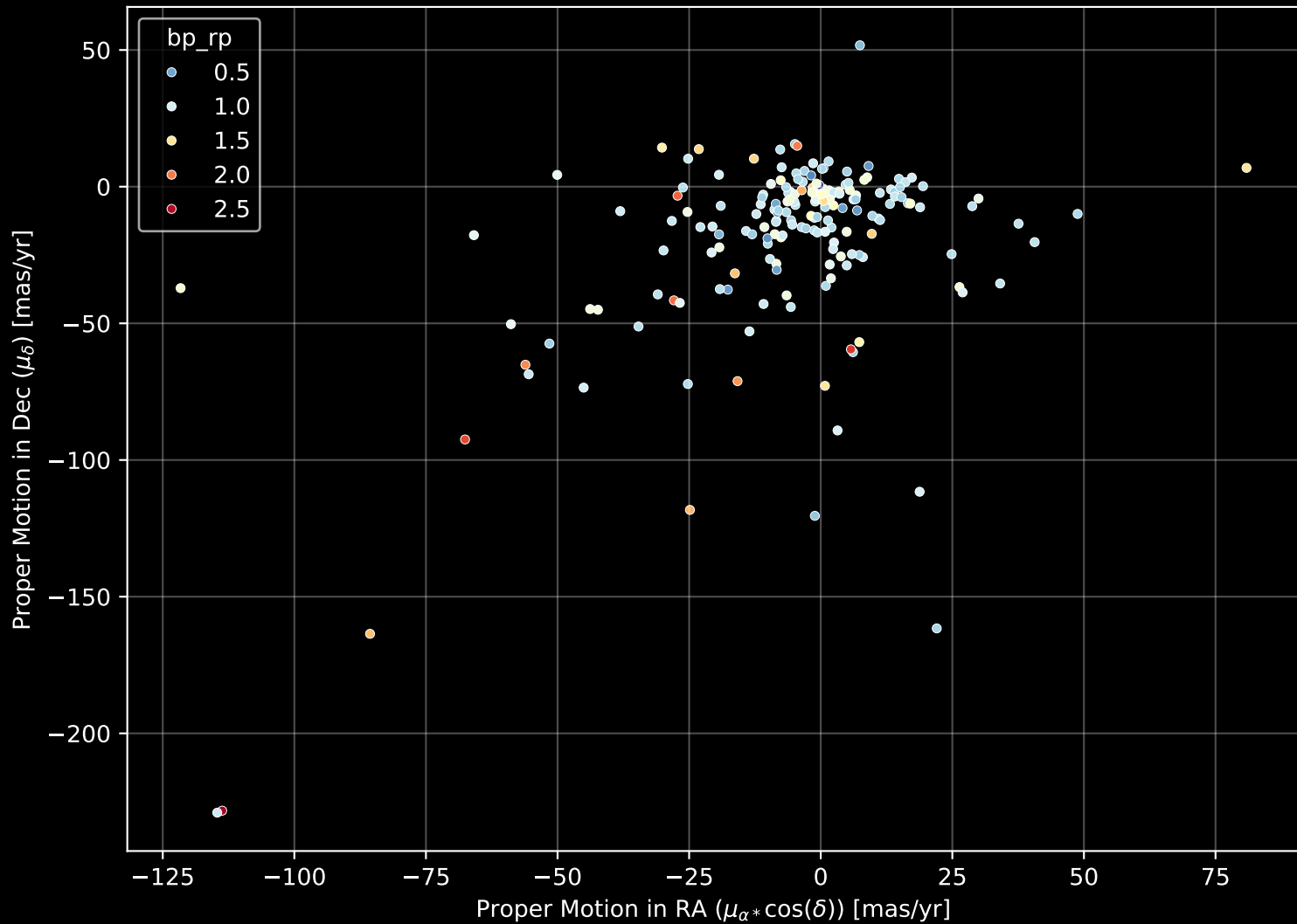
APOGEE DR17 Field: [165+33_MGA] Proper Motion Diagram (n= 187)
