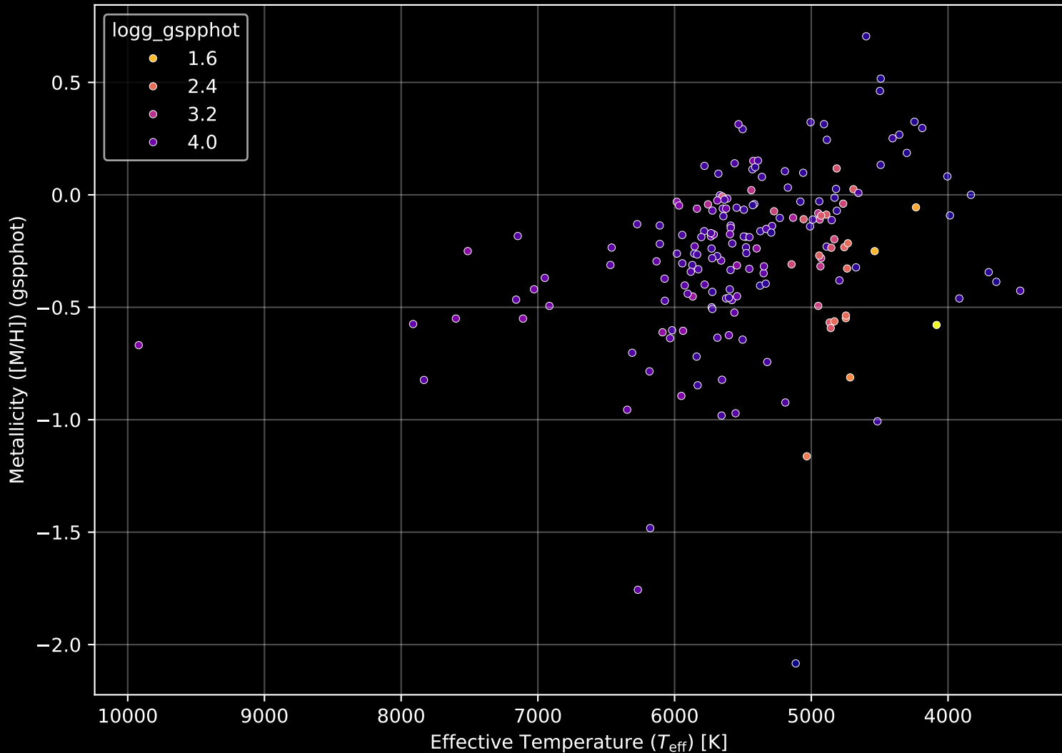
APOGEE DR17 Field: [165+33_MGA] Stellar Population Parameters (n= 187)
