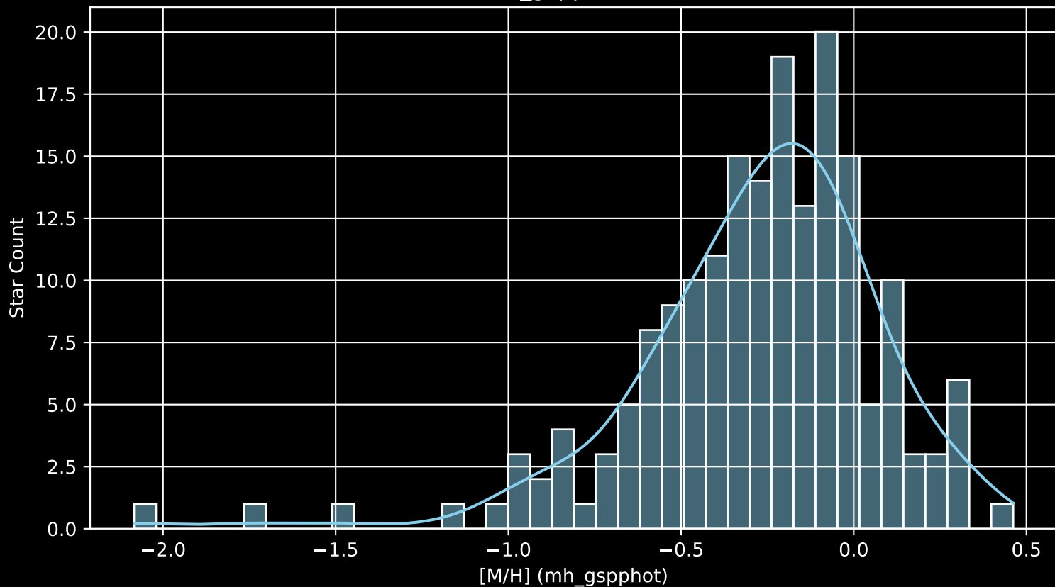
APOGEE DR17 Field: [165+33_MGA [M/H] (mh_gspphot) (n= 185)
