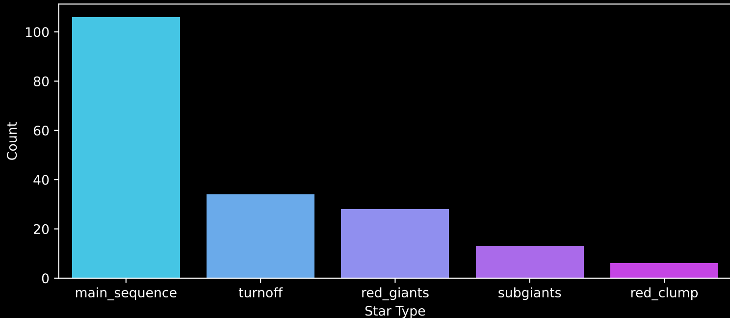
APOGEE DR17 Field: [165+33_MGA] Count plot of Star Type
